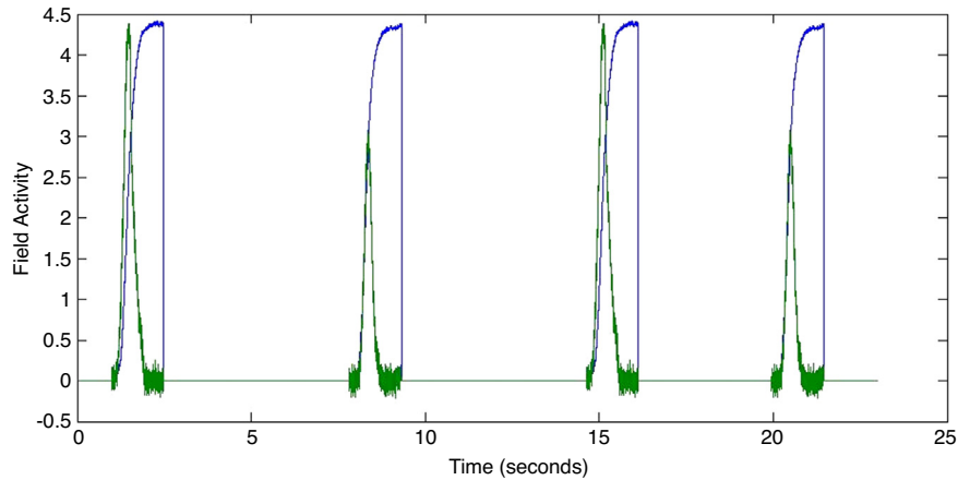
Fig. 7. Excerpted long-form LFP templates computed for two fields in Model 2: fAtn (blue) and go node (green). Depicted is an experimental block of four trials at Load 4, presented to a particular subject in the ordered sequence Go–Nogo–Go–Nogo. (For interpretation of the references to color in this figure legend, the reader is referred to the web version of this article.)
