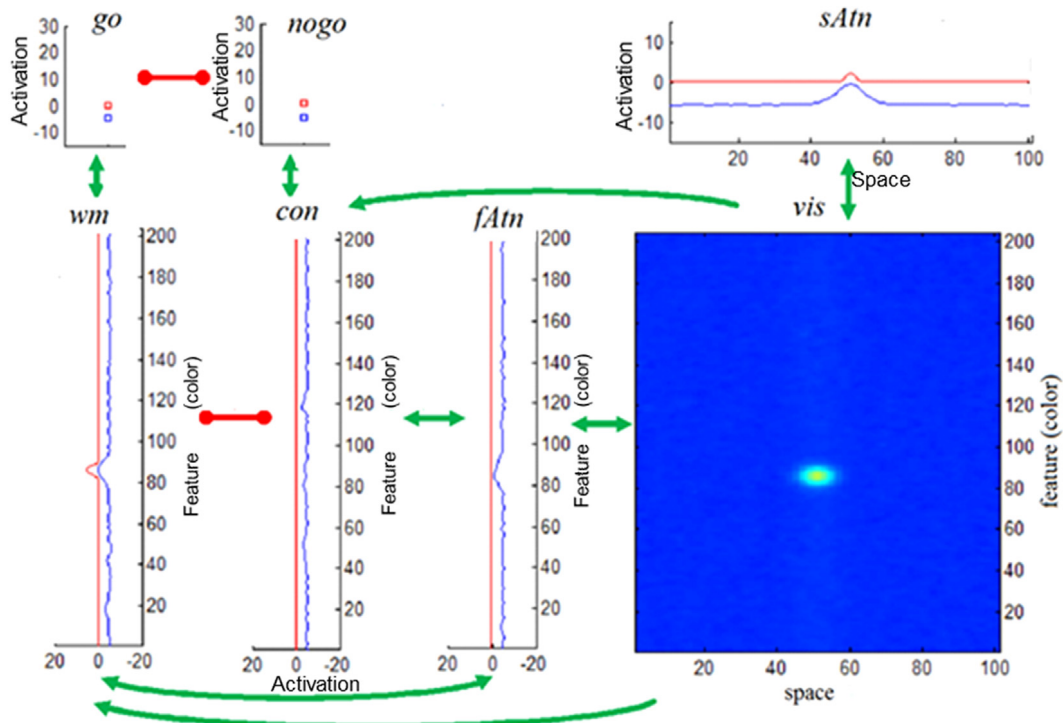
Fig. 2. Architecture of the GnG DNF model. Seven sub-networks are included: (i) the visual field, vis; (ii) the spatial attention field, sAtn; (iii) the feature attention, fAtn; (iv) the contrast field, con; (v) the working memory field; wm; (vi) the go and (vii) nogo nodes. The neural fields are coupled by uni- or bi-directional excitatory (green) or inhibitory (red) connections. Within each field, the activation variable u(x, t) at a given time instance t = \tilde{t} is plotted in blue. Field output g(u(x, t)) at t = \tilde{t} is in red. The range [-20, 20] (horizontal axis for fAtn, con, wm), or [-15, 30] , [-15, 30] (vertical axis for sAtn, go, Nogo) shows values taken by activations and field outputs. Feature (color) and space dimensions have a span of 204 units (vertical axes in the lower panels) and 101 units (horizontal axes in upper and lower right panels) respectively. (For interpretation of the references to color in this figure legend, the reader is referred to the web version of this article.)
