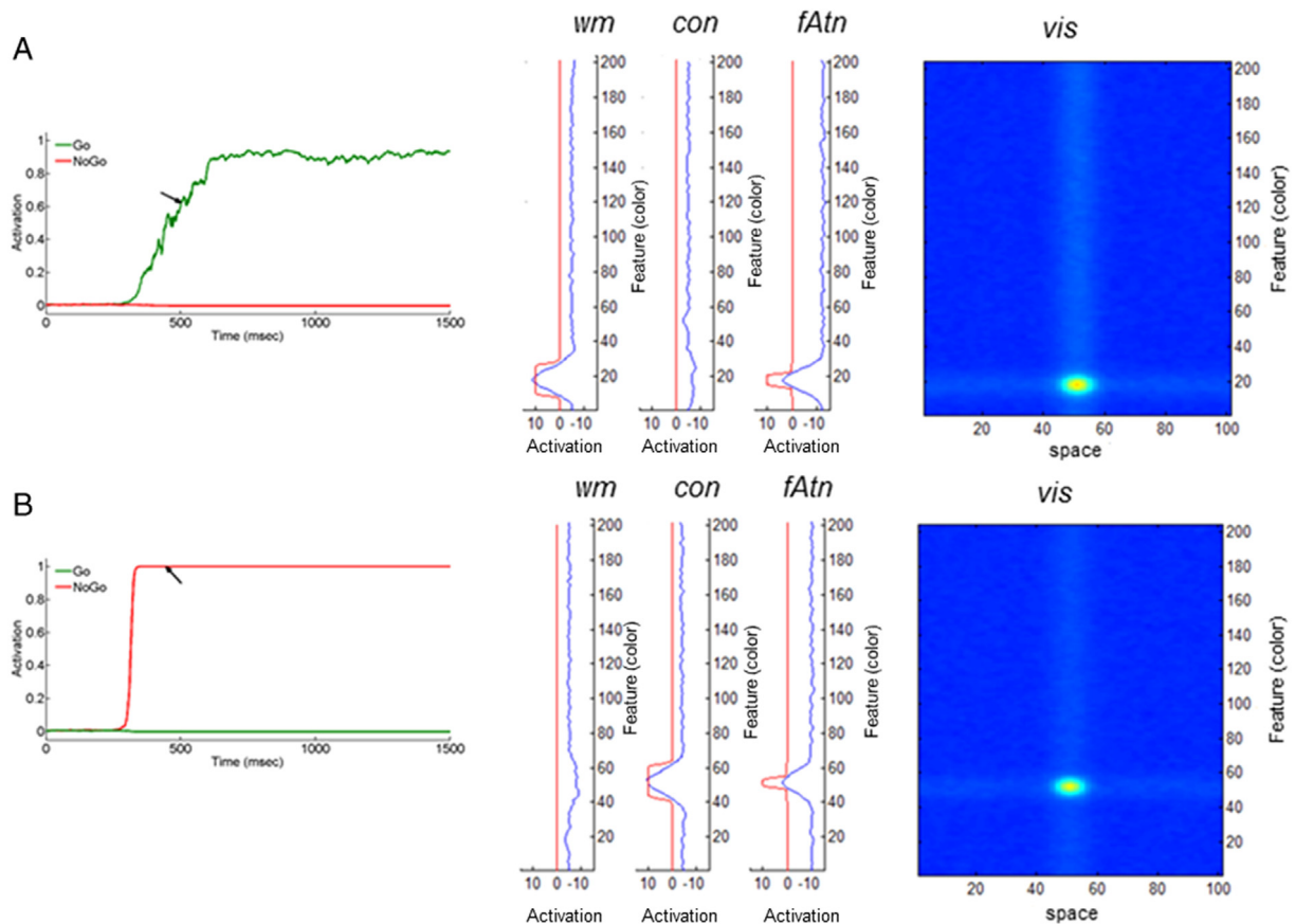
Fig. 3. Network state of the DNF model at time instance \tilde{t} approximately 500 ms after stimulus onset during: (A) Go task and (B) Nogo task (only vis, fAtn, con, wm are shown). Time evolution of the output of go (in green) and Nogo (in red; left panel) nodes is also shown. Time \tilde{t} is indicated by the black arrow. Simulations used parameters from Appendix (see Model 1 and Load 2 condition). (For interpretation of the references to color in this figure legend, the reader is referred to the web version of this article.)
