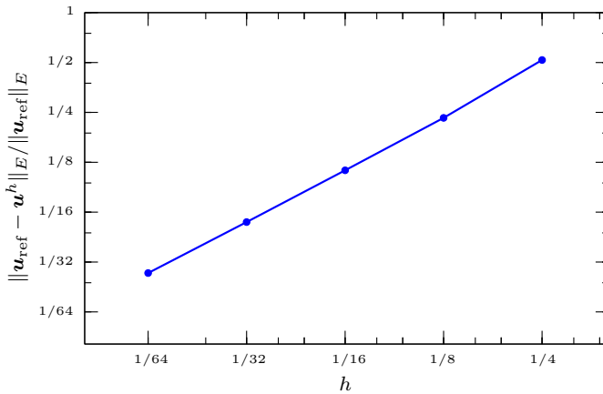
Figure 7.5. Relative errors in energy norm for the second example.
