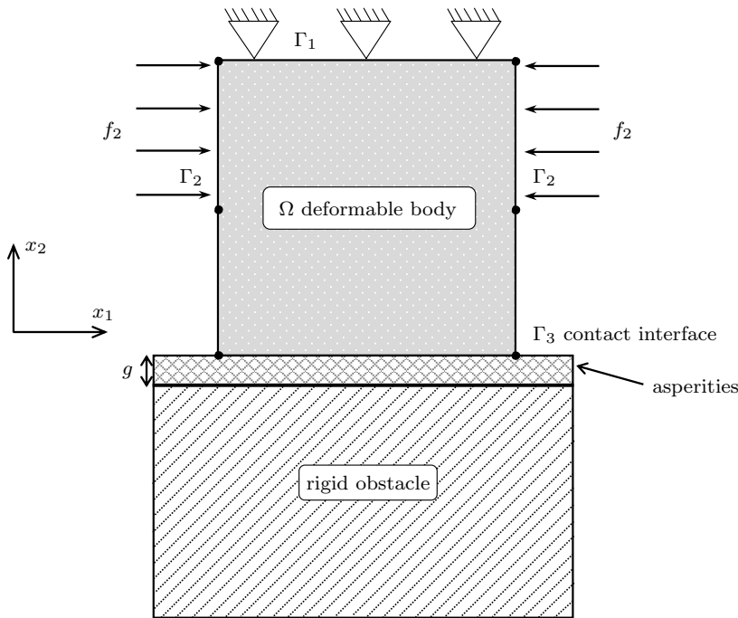
Figure 7.1. Reference configuration of the two-dimensional body.
