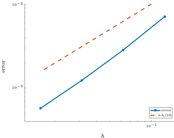
Figure 8.2. Numerical evidence of first-order convergence of \|\mathbf{u}_{\text{ref}}(\cdot, 1) - \mathbf{u}_N^{hk}\|_1 ( N = 1/k ) with respect to h .
