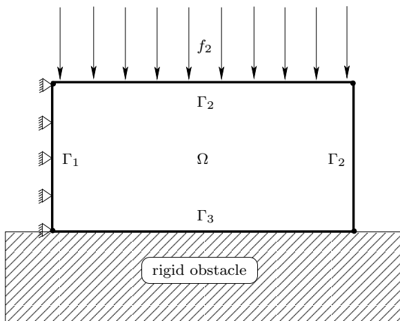
Figure 9.1. Physical setting of the contact problem.
